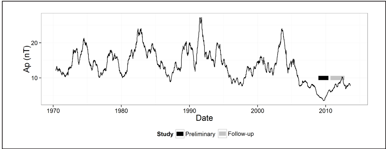
Figure 2. Smoothed index of planetary GMA ( A_p ) from 1970 to 2013. The period of the preliminary study is marked in black, and the follow-up study in grey.
