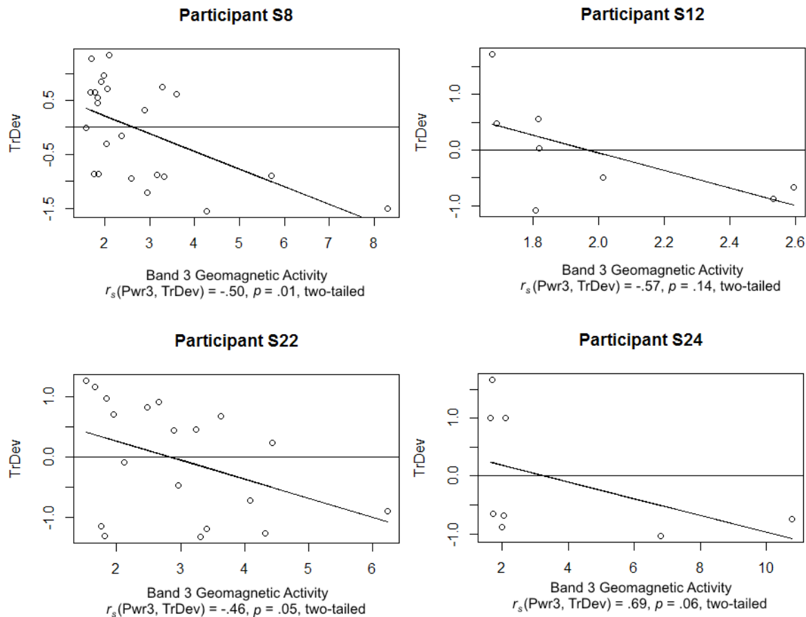
Figure 8. Individual participants' correlation between band 3 GMA and psi score.
