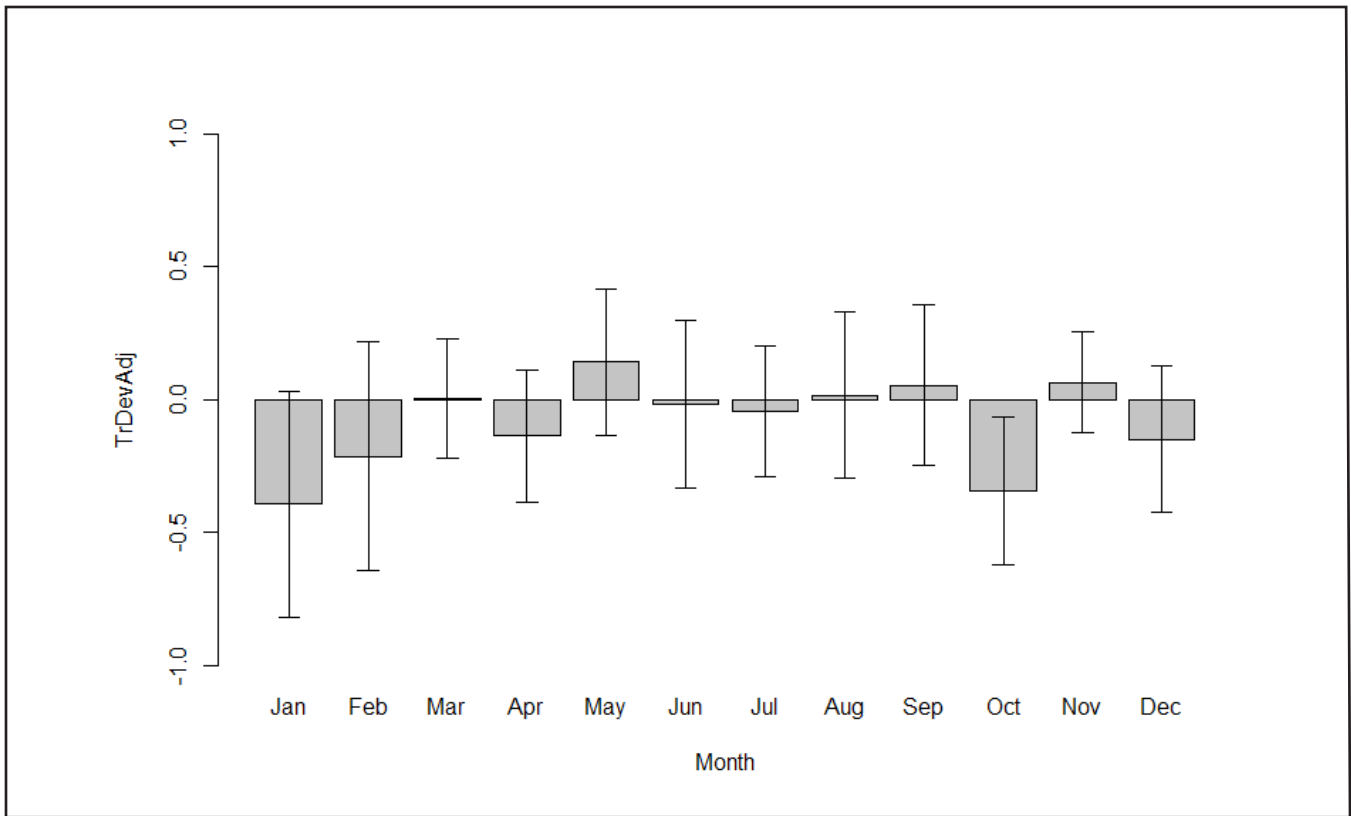
Figure 6. Adjusted Psi score by month, with 95% confidence interval (overall).
