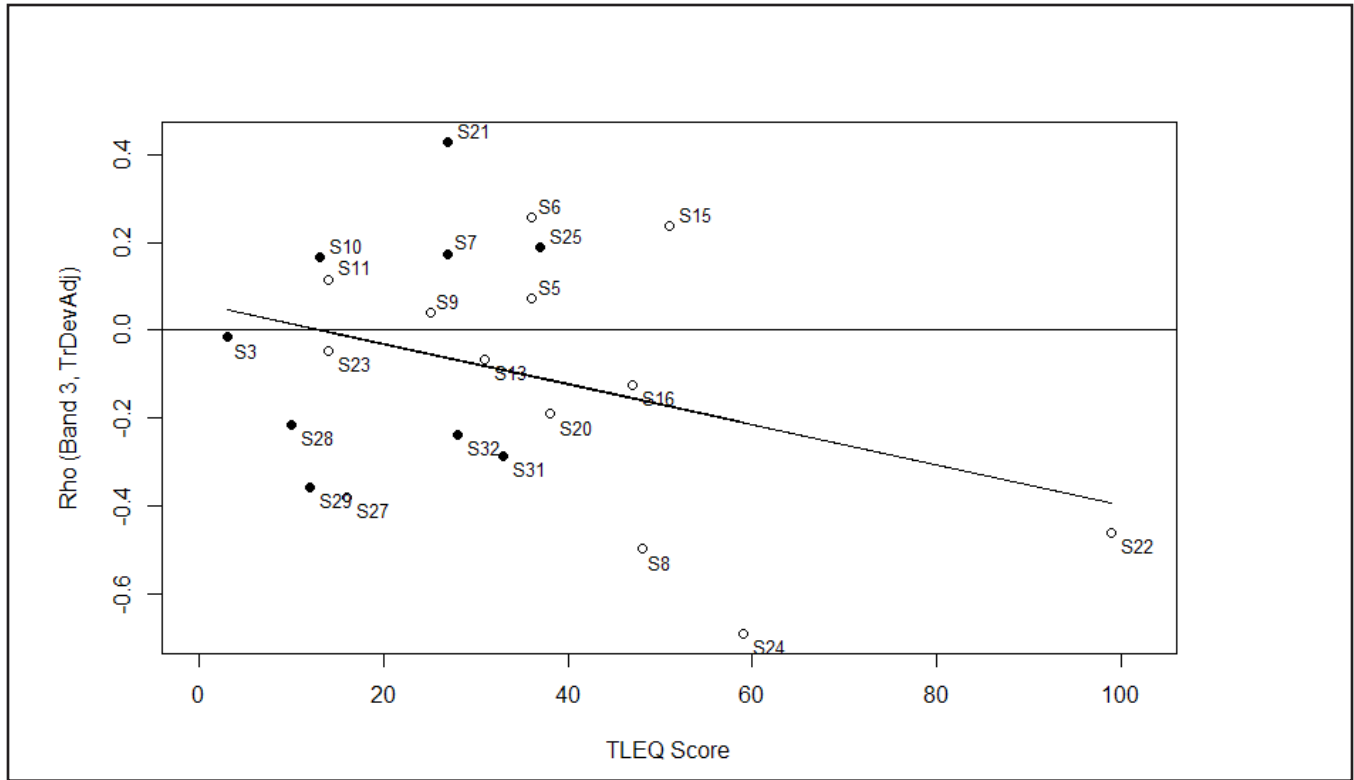
Figure 5. Participants' TLEQ scores (x-axis) vs. correlation between band 3 GMA and psi scoring (y-axis).
