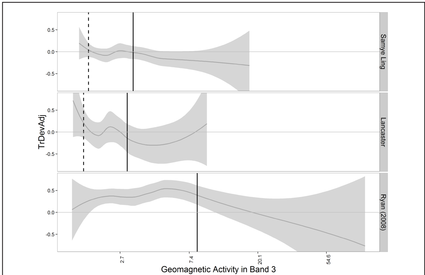
Figure 4. Smoothed mean psi score (TrDevAdj) by band 3 activity (grey line) and 95% confidence interval (grey ribbon). Top panel: Samye Ling (both studies combined); middle panel: 100 remote viewing trials conducted at Lancaster University; bottom panel: 343 free-response trials examined by Ryan (2008), on which the formal hypothesis was based. Solid vertical lines indicate GMA threshold above which psi scoring falls; dashed vertical lines indicate GMA threshold below which psi scoring increases. In Ryan (2008) only one threshold point was used.
