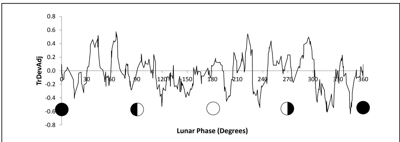
Figure 7. 12-point moving average of psi score by lunar phase (overall).
