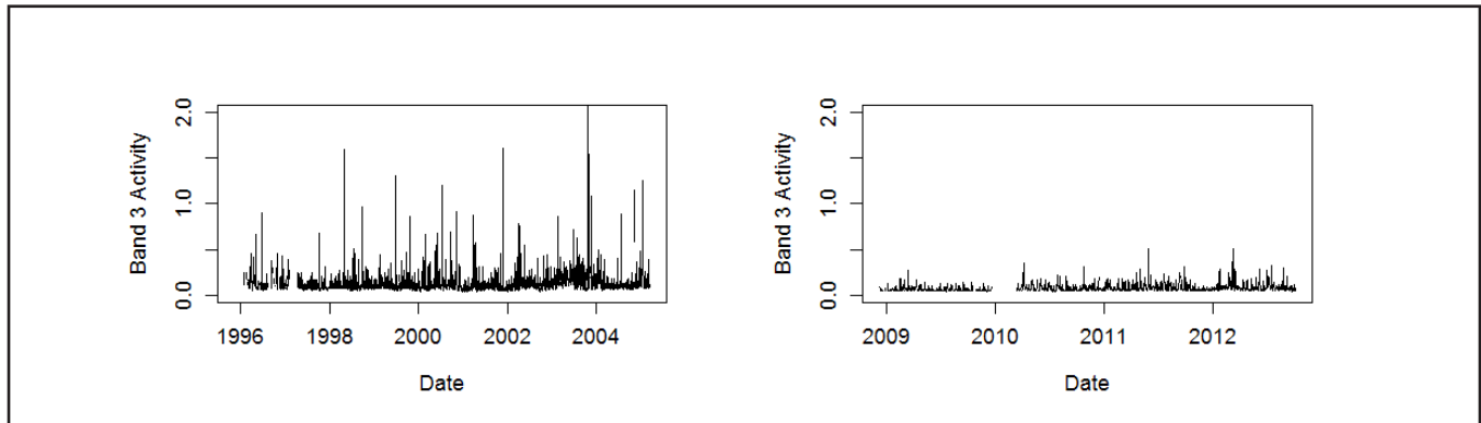
Figure 3. Left: Band 3 GMA during the period studied by Ryan (2008). Right: Band 3 GMA during the period of preliminary and follow-up studies.
